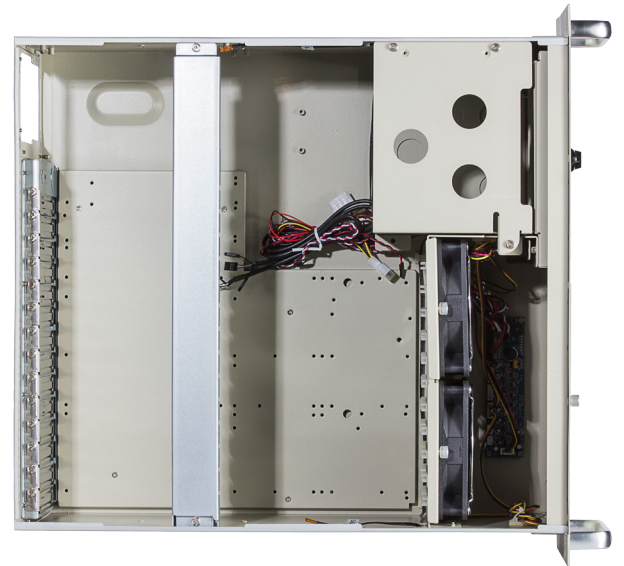
Inside view
